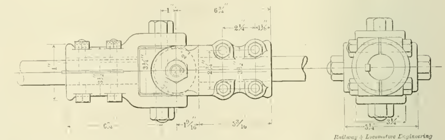
UNIVERSAL COUPLING BETWEEN MOTORS AND MACHINES.
